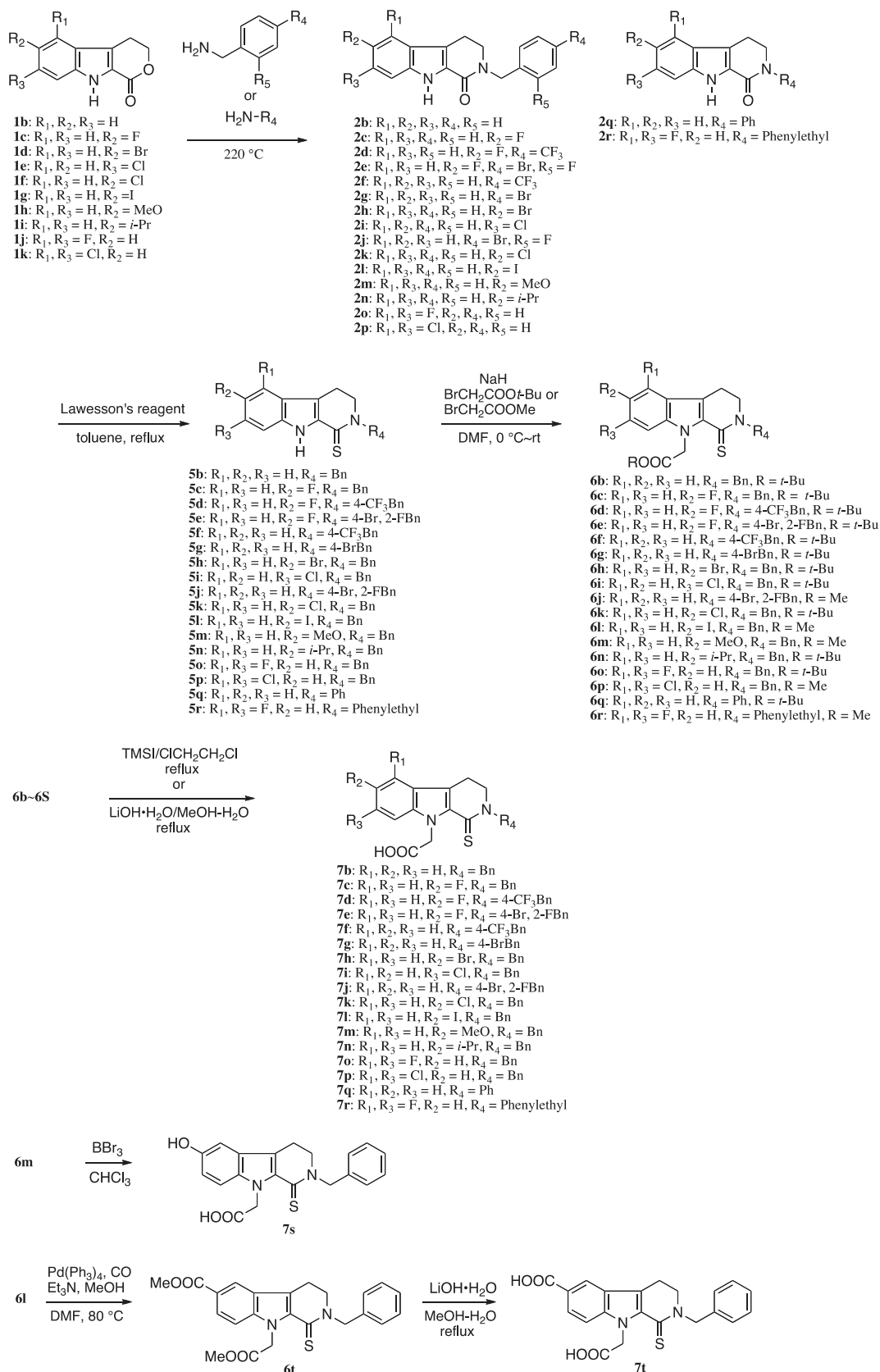
Scheme 2.
